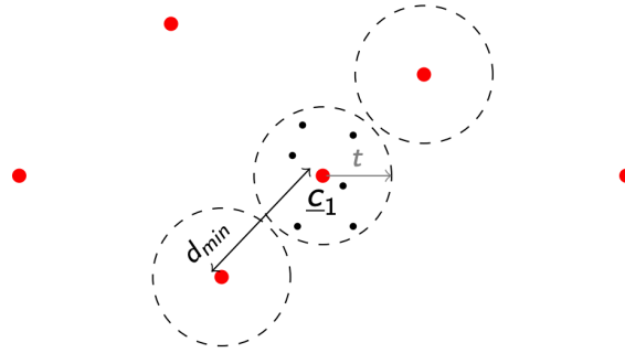
Figure 1: The big dots represent the codewords, the little ones are the other length- n binary sequences
